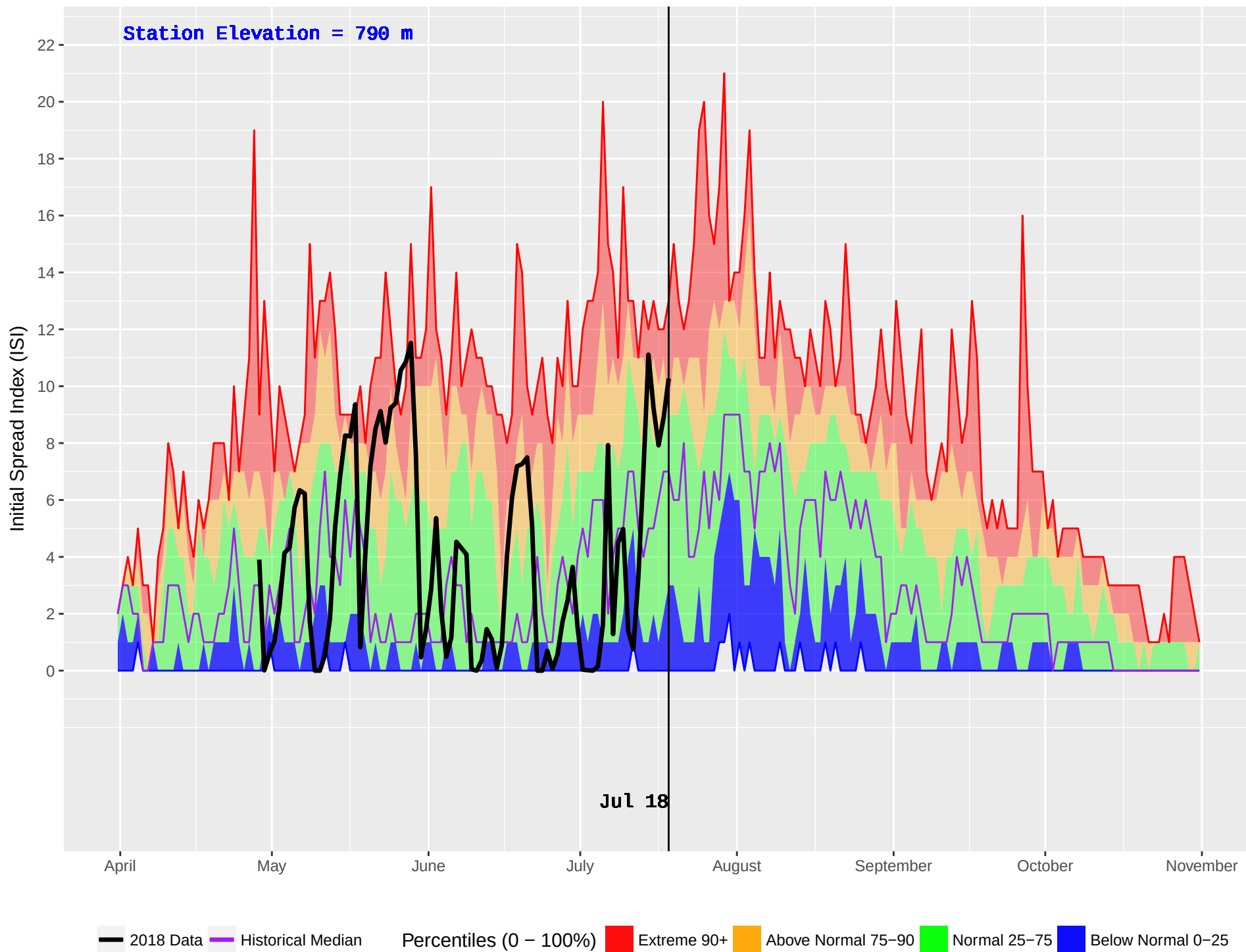
FALLS CREEK (383) : Historical (2002–2016) and Current (2018) Daily Initial Spread Index (ISI)
